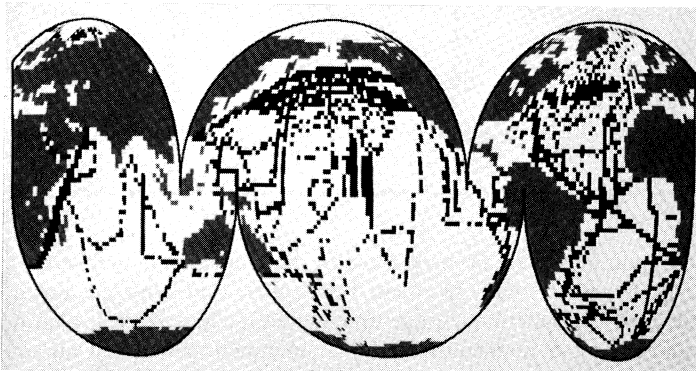
Fig. 2. The distribution of measurements of \Delta p\text{CO}_2 since 1972. Where observations were made quasi-continuously, the values have been averaged over 2° intervals in longitude and latitude, and each of these intervals is represented by a single dot on the map.
