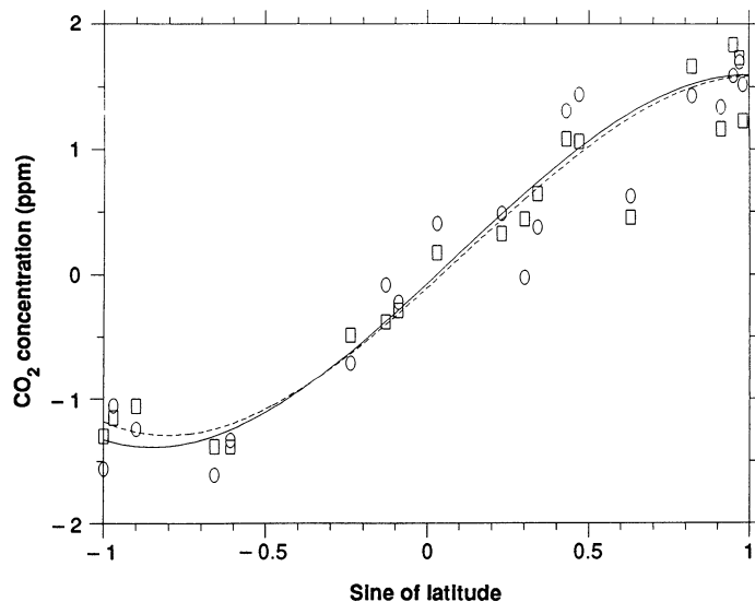
Fig. 5. Results of model calculations (scenario 1, Table 3) of the atmospheric \text{CO}_2 concentrations at the GMCC sites (squares and dashed curve) are compared with the observed concentrations (circles and solid curve). All values are relative to the global mean. The curves are least-squares cubic polynomial fits; the differences between the curves are not statistically significant.
