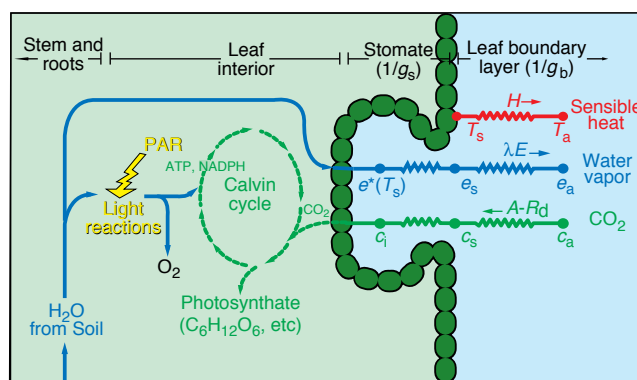
Fig. 3. Schematic of carbon and water exchange in a leaf as conceptualized in a combined photosynthesis-conductance model (39, 40, 42, 43). The stomatal conductance ( g_s ) is a direct function of photosynthesis, \text{CO}_2 concentration at the leaf surface ( c_s ), and relative humidity at the leaf surface [ h_s = e_s/e^*(T_s) ; e_s = vapor pressure at leaf surface] (see Eq. 7).
