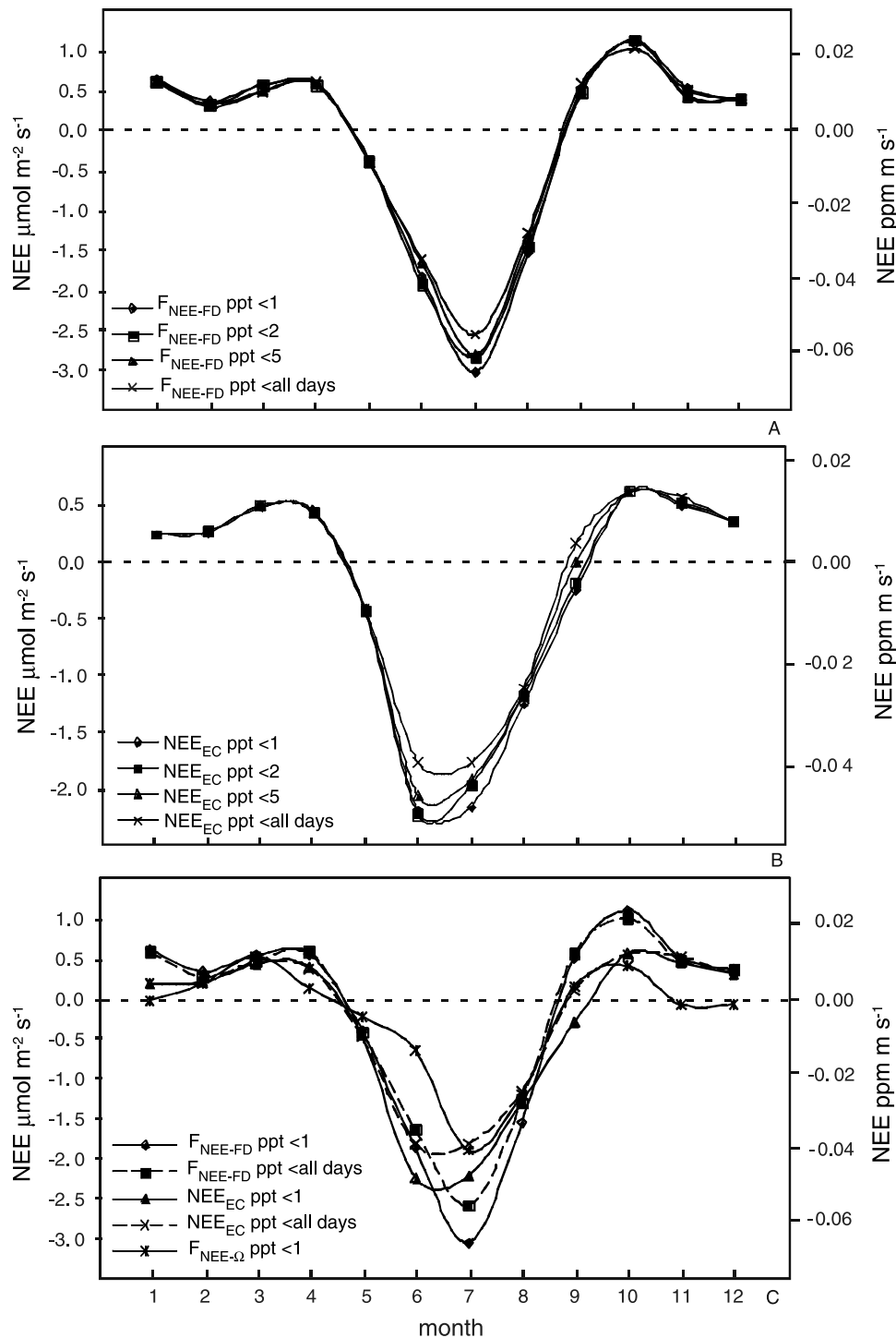
Figure 5. Net ecosystem exchange for CO 2 (NEE) (a) as determined by equation (1) ( F_{NEE-FD} ) and using the \rho W estimates from Figure 3 and (b) from eddy covariance estimates for all days in a month and with precipitation filters ppt < 1, 2, and 5 mm applied. (c) F_{NEE} determined by the reanalysis-2 data derived \rho W_{\Omega} ( F_{NEE-\Omega} ) for ppt < 1 is presented with NEE_{EC} and F_{NEE-FD} for direct comparison of estimates. See color version of this figure in the HTML.
