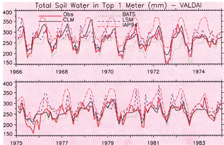
FIG. 2. Simulated and observed soil moisture in the top 1 m for the end day of each month for 1966–83 for the Valdai catchment. The observational values represent catchment-averaged soil water measured by the gravimetric method at the end of each month from 9 to 11 sites distributed over the catchment (Vinnikov et al. 1996).
