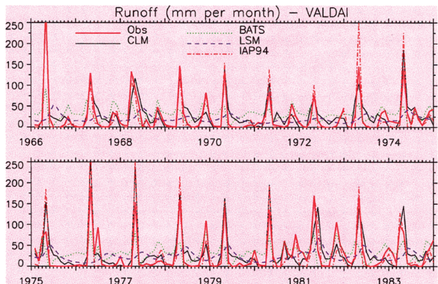
FIG. 3. Monthly mean simulated and observed runoff for 1966–83 for the Valdai catchment. Monthly runoff measurement were obtained by weir observations made at the outflow point of the catchment region (Schlosser et al. 1997).
