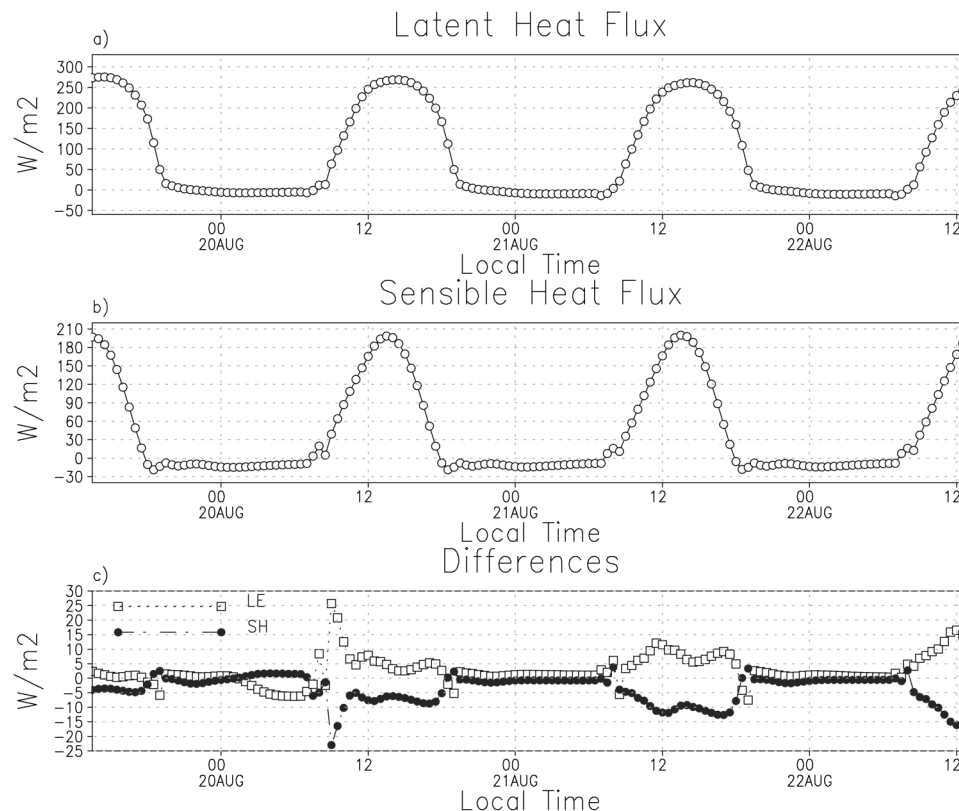
Figure 4. Temporal evolution of the latent (a) and sensible (b) heat fluxes in the lowest atmospheric model level for the control case and the difference (c) given by the enhanced entrainment case minus the control case.
