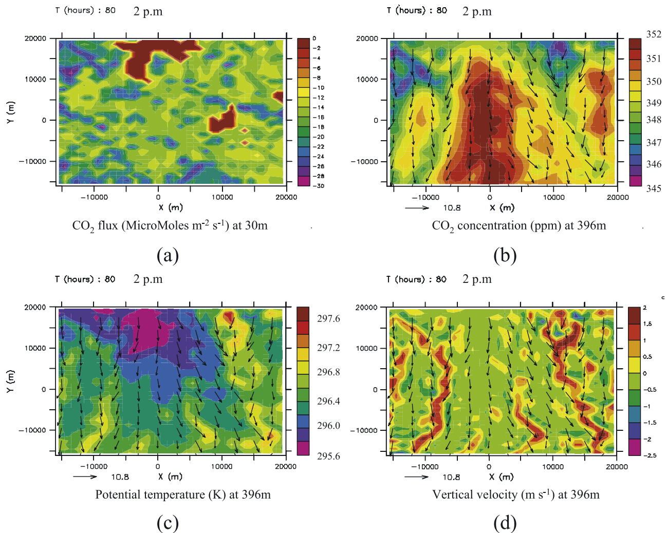
Figure 8. Horizontal cross sections of (a) \text{CO}_2 flux ( \text{micromoles m}^{-2} \text{s}^{-1} ) at 30 m and (b) \text{CO}_2 concentration (ppm), (c) potential temperature (K), and (d) vertical velocity ( \text{m s}^{-1} ) at 396 m for grid 3 at t = 80 h (2 p.m. LST).
