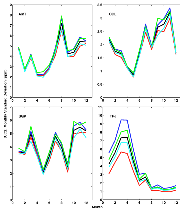
Fig. 9. Comparison of monthly standard deviation of mid-afternoon CO 2 from VERTMIX experiments (color) to CONTROL simulation (black) at grid cells containing AMT (top left), CDL (top right), SGP (bottom left), and TPJ (bottom right). VERTMIX experiments include half_cmf (blue), twice_cmf (red), half_vdif (green), and twice_vdif (cyan).
