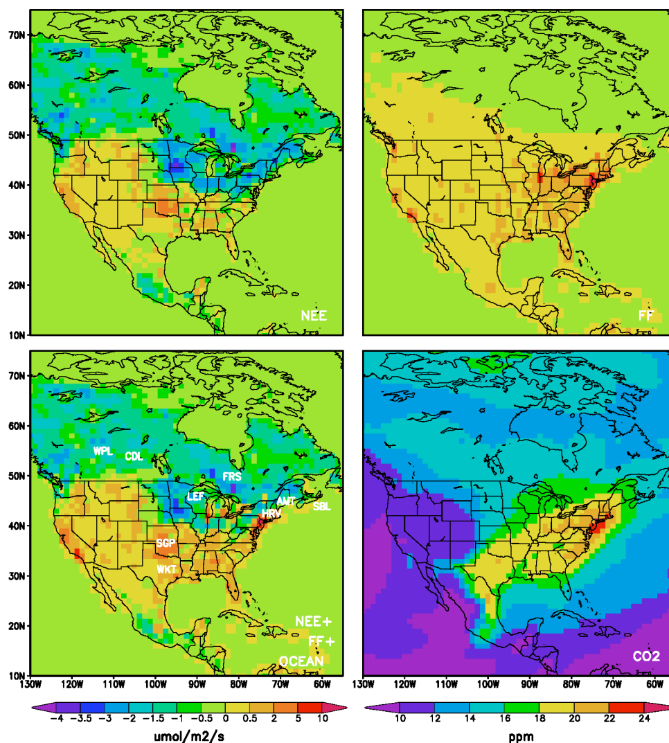
Fig. 6. July mean surface CO 2 flux of net ecosystem exchange (NEE, top left), fossil fuel emissions (FF, top right), total surface flux (NEE + FF + air-sea exchange (OCEAN), bottom left), and boundary layer CO 2 (bottom right) for North America. Plots of surface flux are on the same scale, with units of \mu\text{mol}/\text{m}^2/\text{s} , corresponding to the color bar on the bottom left. CO 2 is plotted in units of ppm, with the corresponding color bar on the bottom right. Locations of continuous sites are plotted in the bottom left plot for convenience.
