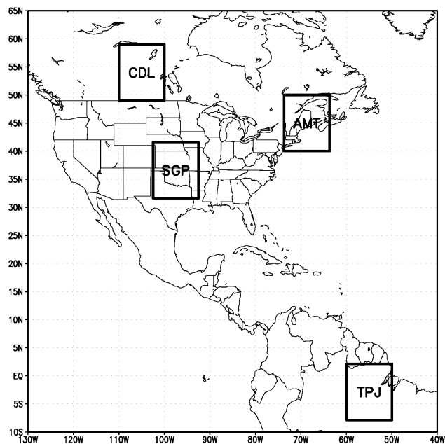
Fig. 7. Domains used for NOFLUX, NOCONV, and RADCLIM sensitivity experiments. Grid cells at the center of each domain are used for analysis. The same grid cells are used in analysis of the VERTMIX experiment.
