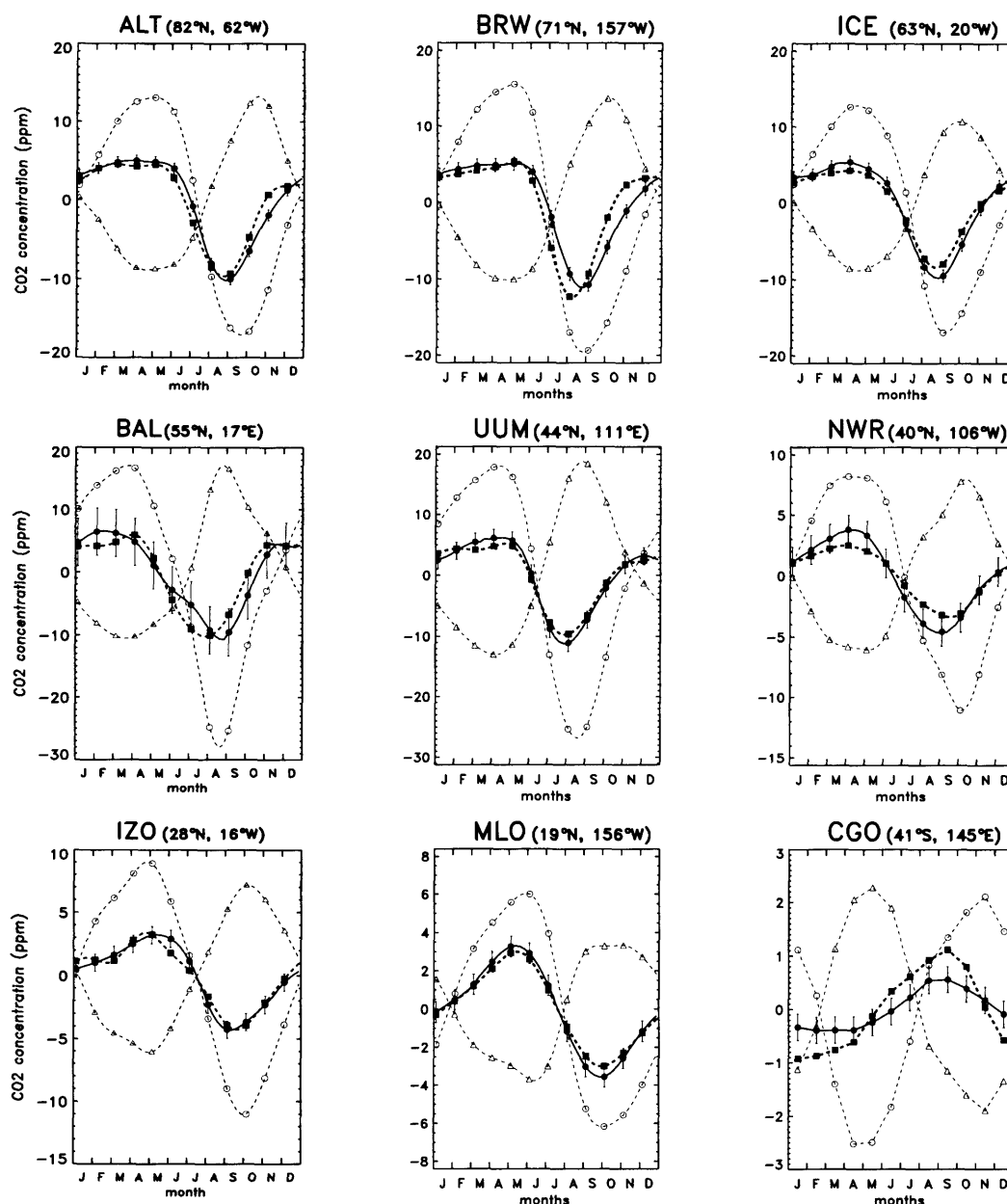
Fig. 1. Mean seasonal cycle of atmospheric \text{CO}_2 concentration, simulated by the TM2 model at a few stations (dashed line) compared with the observations (solid line with circles). Curve with plain squares represents the overall modeled \text{CO}_2 concentration including all processes. Curves with circles and triangles separate the exchange of \text{CO}_2 due only to photosynthesis and respiration, respectively. All curves have been detrended separately as described in Subsection 3.1. (Increase of the photosynthetic curve during winter-time comes only from the detrending process; same for the decrease of the respiration curve.) Error bars on the observations represent \pm the standard deviation of all residuals between flask data and the fitted curve.
