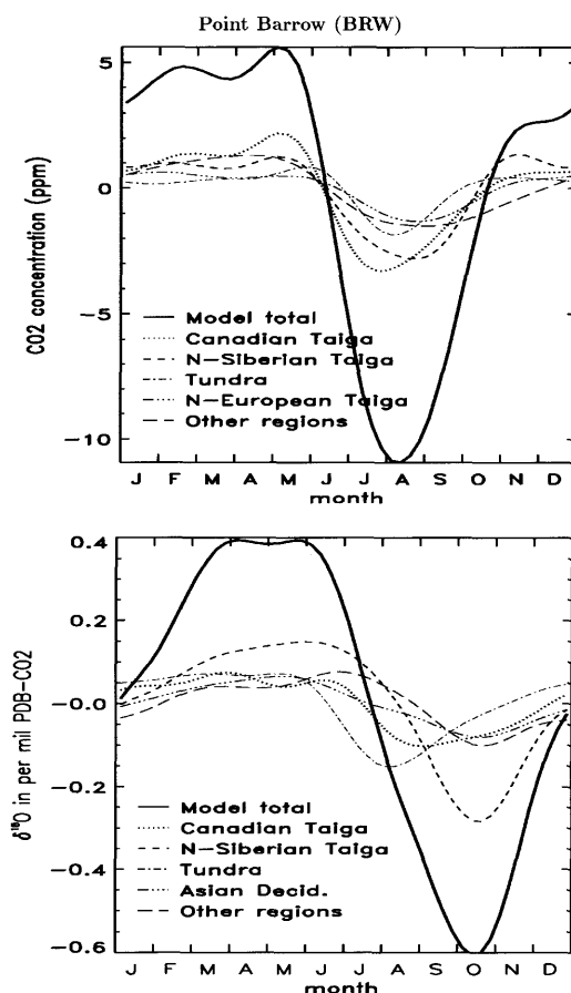
Fig. 6. Simulated mean seasonal cycle (detrended model output) at Point Barrow (BRW) for atmospheric CO 2 (upper graph) and for \delta^{18}\text{O} in atmospheric CO 2 (lower graph). Solid thick line correspond to the overall model simulation including all processes (terrestrial biosphere, ocean, fossil fuels and deforestation). Thin curves separate the contribution of specific land regions (Fig. 5) to the overall seasonal cycle. Regions with low contribution are brought together into one component "other regions" (see Table 2 for the value of each contribution).
