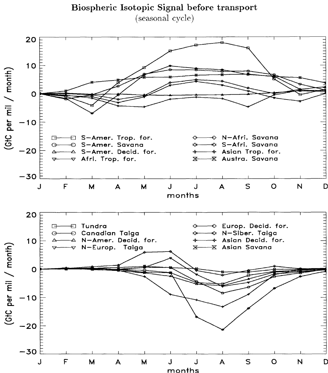
Fig. 8. Seasonal variations of the flux of \delta^{18}\text{O} in atmospheric \text{CO}_2 (in \text{GtC}\text{‰ month}^{-1} ) from 16 land ecosystems (Fig. 5), before atmospheric transport. Values represent the overall contribution of photosynthesis and respiration ( A\Delta_A + F_{\text{resp}}\Delta_R , eq. (A3)). All curves are shifted to zero in January as we will only discuss the seasonality of the fluxes.
