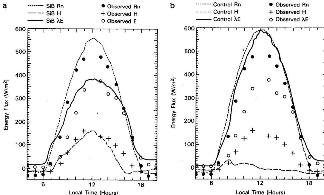
FIG. 2. (a) 30-day (15 June–14 July) mean surface energy balance at Manaus (3°S, 59°W) simulated by SiB and as observed by Shuttleworth et al. (1984a). The lines on the figure represent simulation, the points (circles and crosses) represent the means of observations taken from a site at 30 km from Manaus, Brazil. (b) As in Fig. 2a, except that the simulation was performed by Ctl-GCM.
